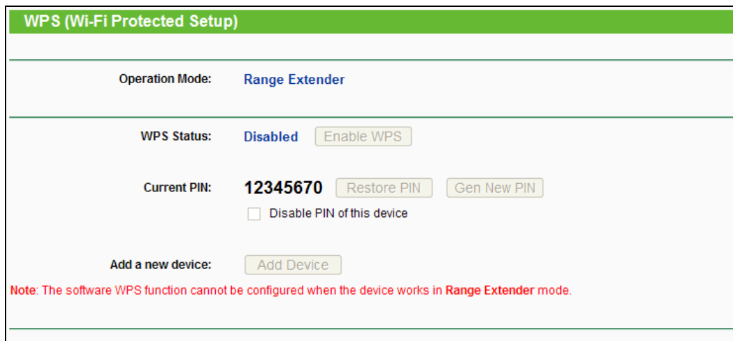
Figure 4-2 WPS – Disabled
